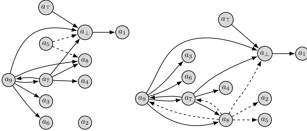
Figure 1: Part of the frameworks from Example 1. In both frameworks \mathbf{A} = \{\text{DDef}, \text{ConUcut}\} . On the left side \mathcal{S} = \{q, \neg p \vee \neg q, r\} and \mathcal{X} = \{p\} , on the right side \mathcal{S} = \{p, q, \neg p \vee \neg q, r\} and \mathcal{X} = \{\} . The dashed arrows denote the differences between the two frameworks.
