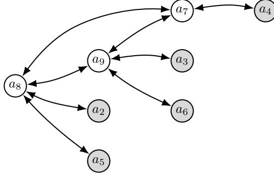
Figure 5: The argumentation framework for Example 11. Highlighted is a stable extension with inconsistent support.
