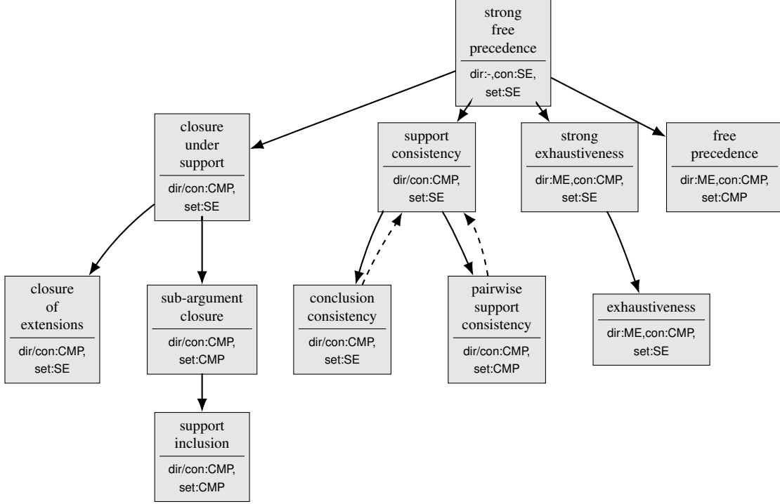
Figure 4: Some relations between the postulates for individual extensions in our setting. If a property at the origin of an arrow in the diagram holds relative to classes of argumentation frameworks for a given semantics \text{sem} and a given attack type \dagger \in \{\text{dir}, \text{con}, \text{set}\} , then also the property at the end of the same arrow holds (for the specified semantics and attack type). For the dashed arrows sub-argument closure, resp. closure under support, is supposed. In each node label, the lower part indicates for which combinations of attack types \dagger and semantics \text{sem} the property holds (as is proved in the propositions in this section).
