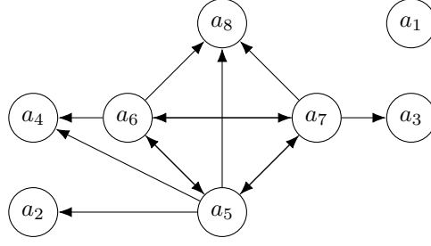
Figure 6: A representation of the framework of Example 6. Note that the argument a_8 with conclusion \neg p does not directly defeat arguments that contain p as a support (such as a_1, a_3 , etc.), since p is a strict assumption.
