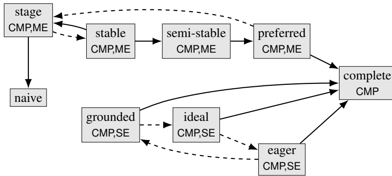
Figure 3: Semantics, their classes, and inclusion relations among them. Strict lines indicate inclusion relations that hold in general and dashed arrows indicate additional relations that hold in the logic-based setting.
