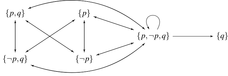
Figure 1: An attack diagram for Example 2
