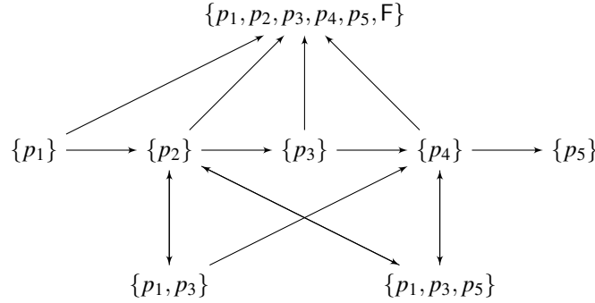
Figure 4: An attack diagram for Example 14
