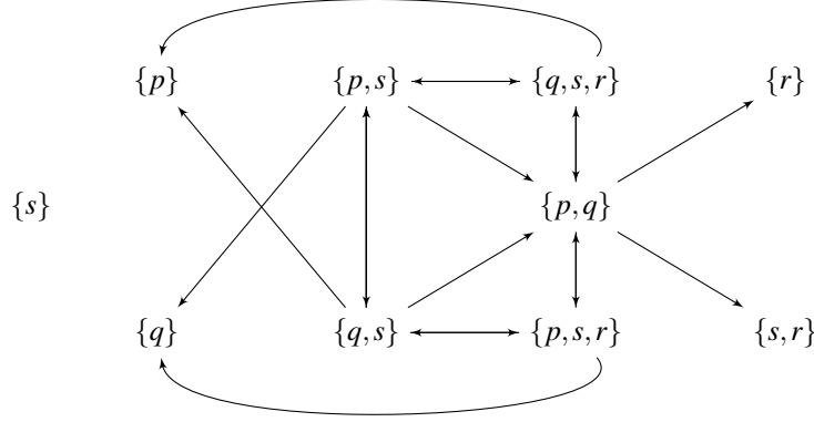
Figure 3: An attack diagram for Example 13
