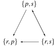
Figure 5: An attack diagram for \text{pABF}' in Example 19
