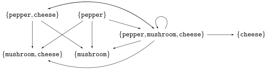
Figure 2: An attack diagram for Example 10
