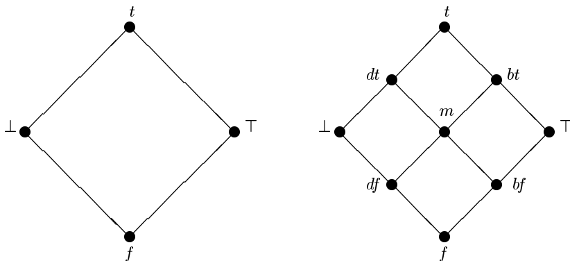
Fig. 1. \mathcal{FOUR} and \mathcal{NLNE}
