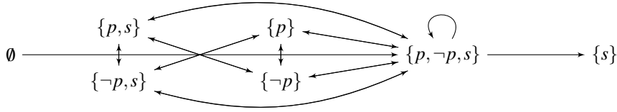
Figure 3. An attack diagram for Example 5
