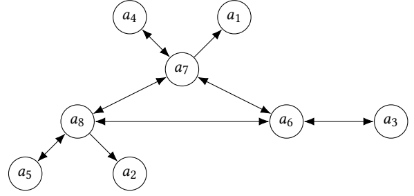
Figure 1: Part of the sequent-based argumentation graph for \mathcal{S} = \{p, q, \neg p \vee \neg q\} from Example 2.6
