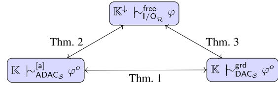
Figure 5: Equivalences for defeasible normative reasoning.
