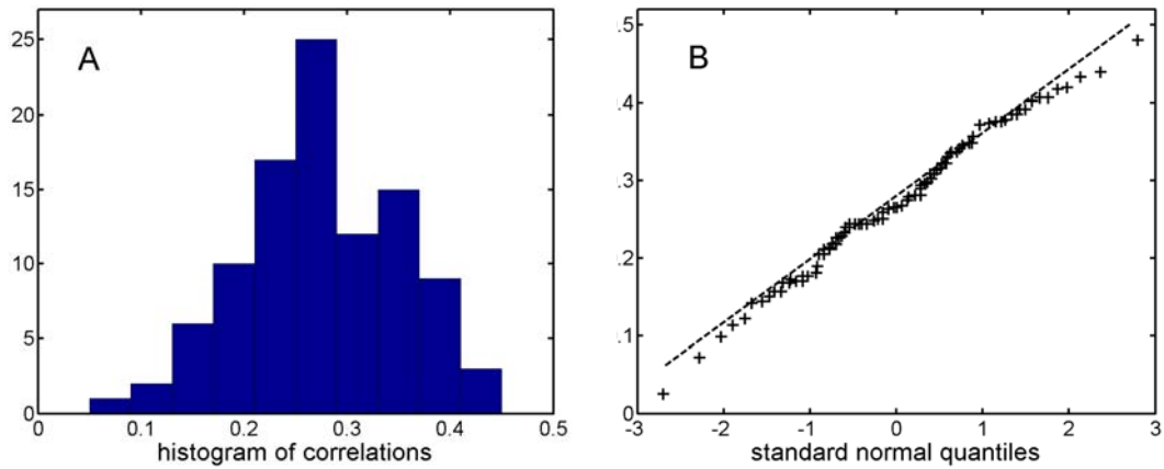
Figure 6: Correlations achieved with random ratings: (A) Histogram of correlations; (B) QQplot of correlations vs. standard normal distributed data. Correlations were obtained with KNN predictor.
