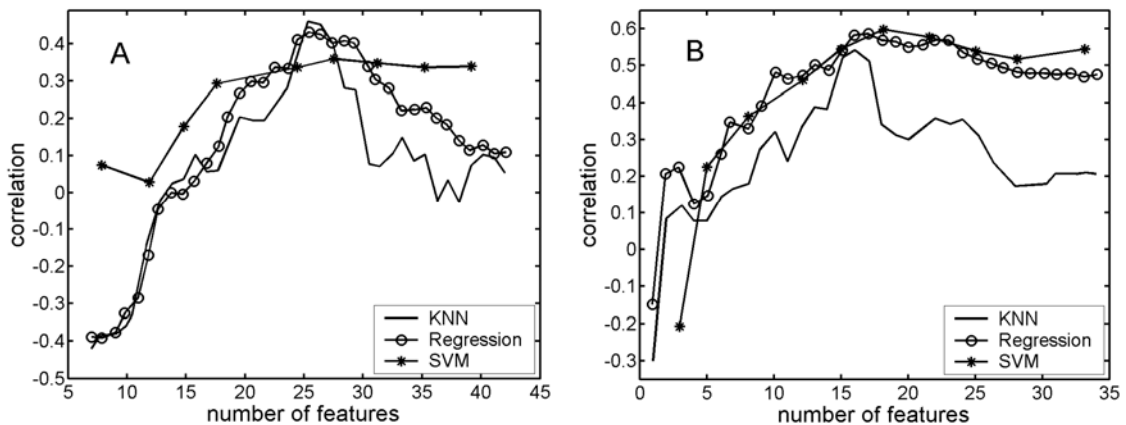
Figure 5: Prediction results obtained with pixel images (A) and with feature-based representation (B). Performance is measured by the correlation between the predicted ratings and the human ratings.
